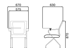
CE/CAL, CE/CA ( W575 x D630 x H870 )
